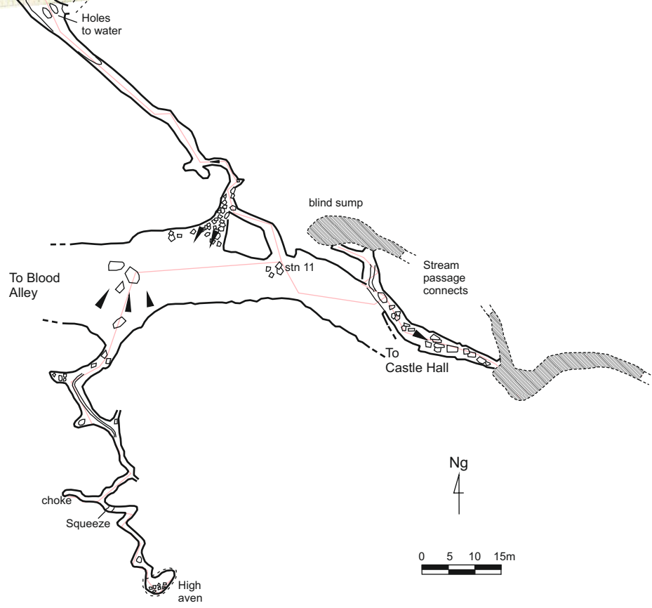
0048 Cueva-Cubío de la Reñada Breakdown Chamber-Squirrel's Passage Surveyed 1982, 2010, 2011 and D Ryall 2009
